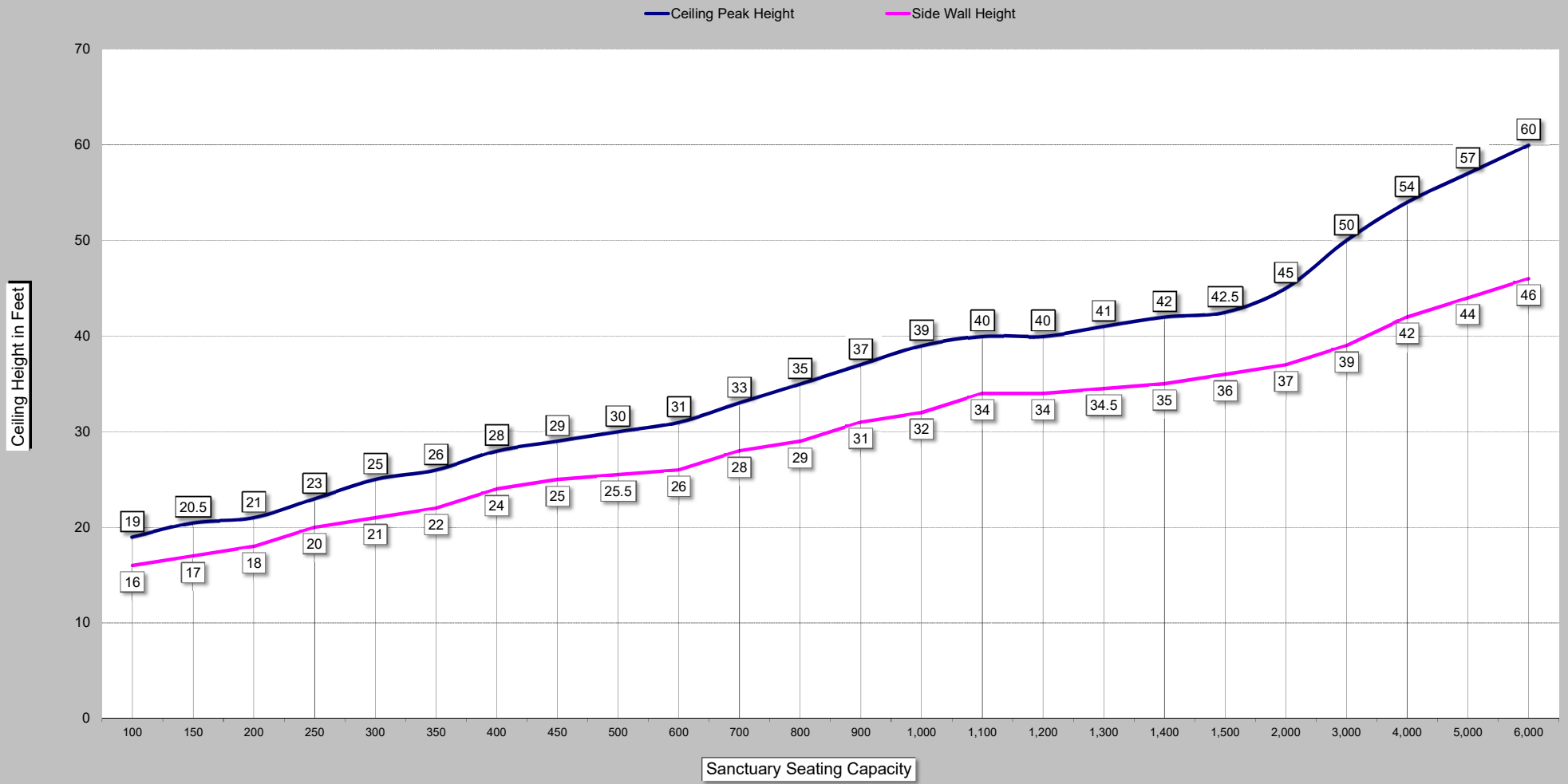
Minimum Church Height Chart
